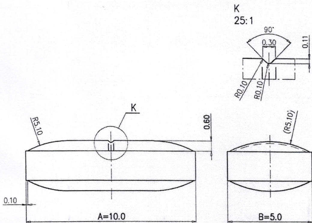
Upper punch side view
